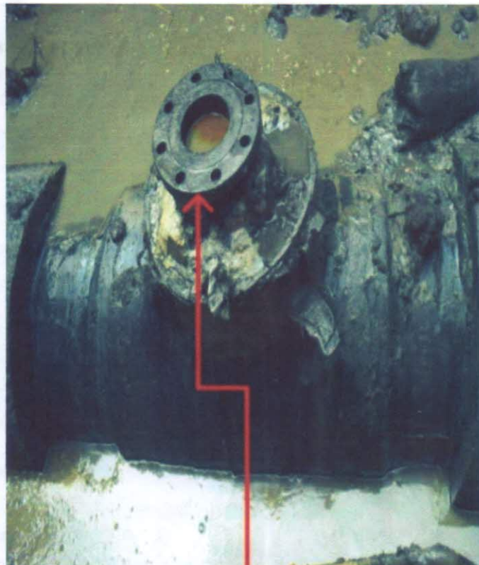
4" NIPPLE VALVE INSTALLED BY VANDALS
